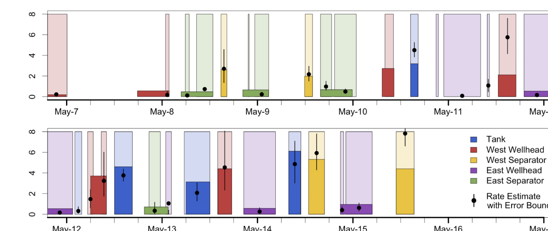
Figure 3: Detection, localization, and quantification results over a selected period from May 7 to May 16, 2022.
