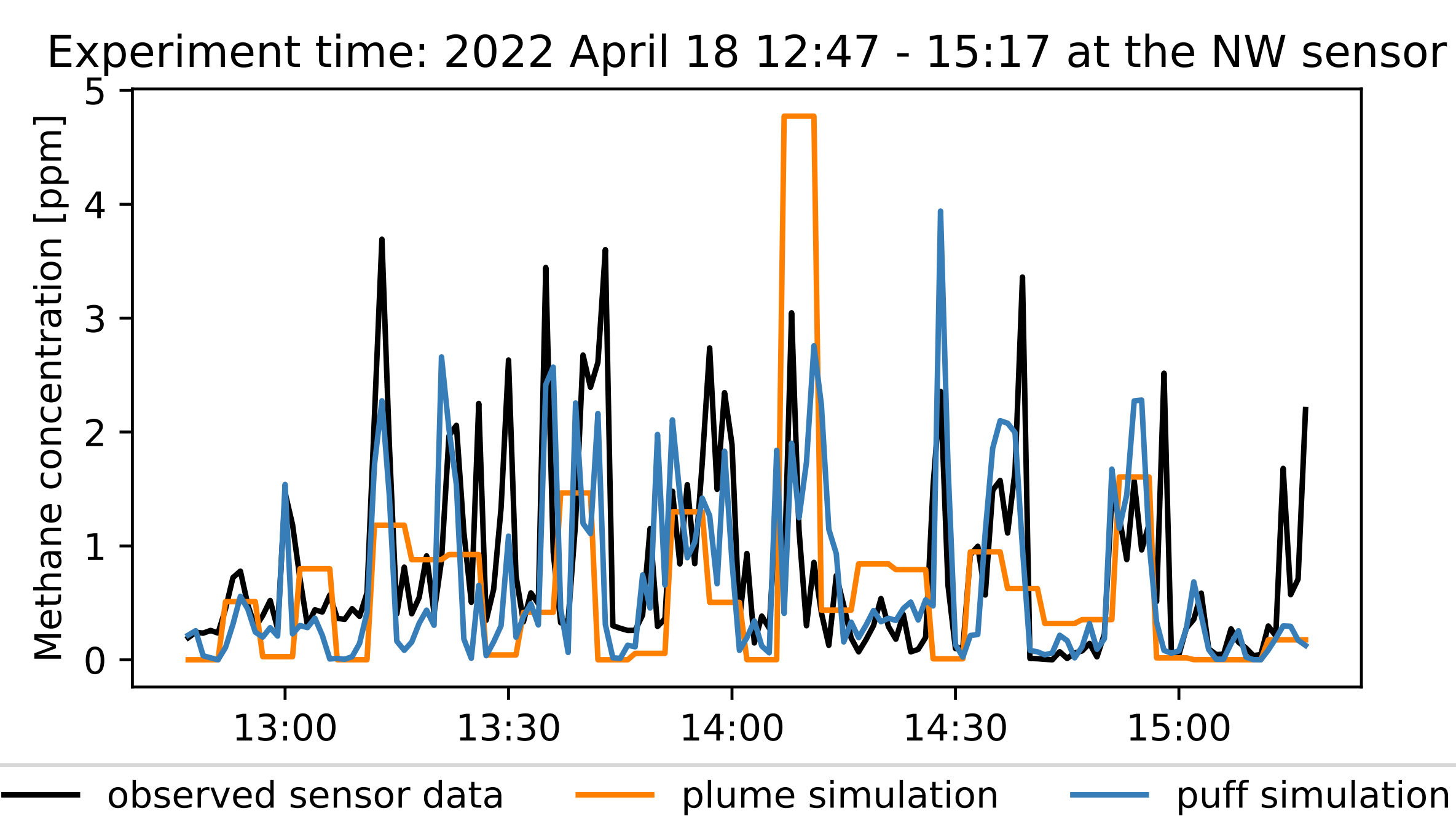
Figure 2: A comparison of simulation predictions from the Gaussian plume and puff models.
