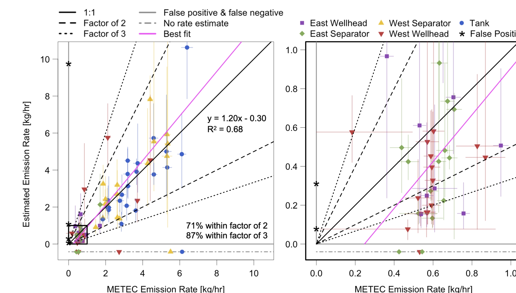
Figure 5: Parity plots of true and estimated emission rates.
