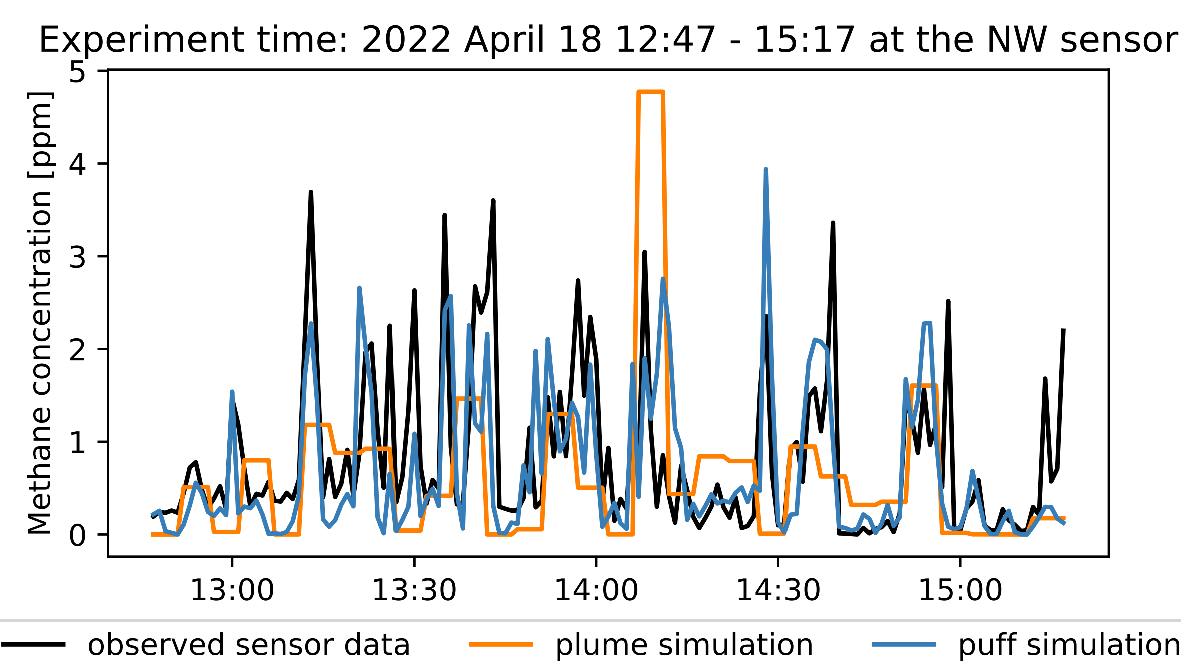
Figure 2: A comparison of simulation predictions from the Gaussian plume and puff models.
